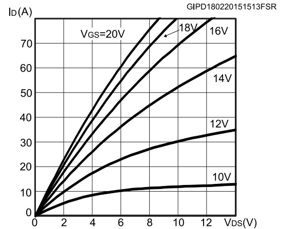
Figure 5: Output characteristics ( T_J = 150^\circ C )
