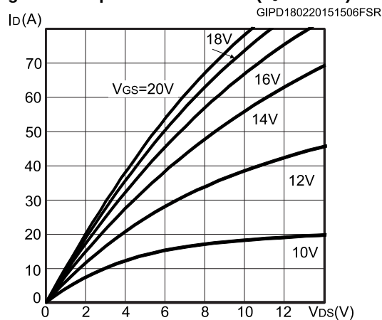
Figure 6: Output characteristics ( T_J = 200^\circ C )
