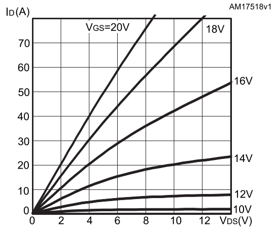
Figure 4: Output characteristics ( T_J = 25^\circ C )
